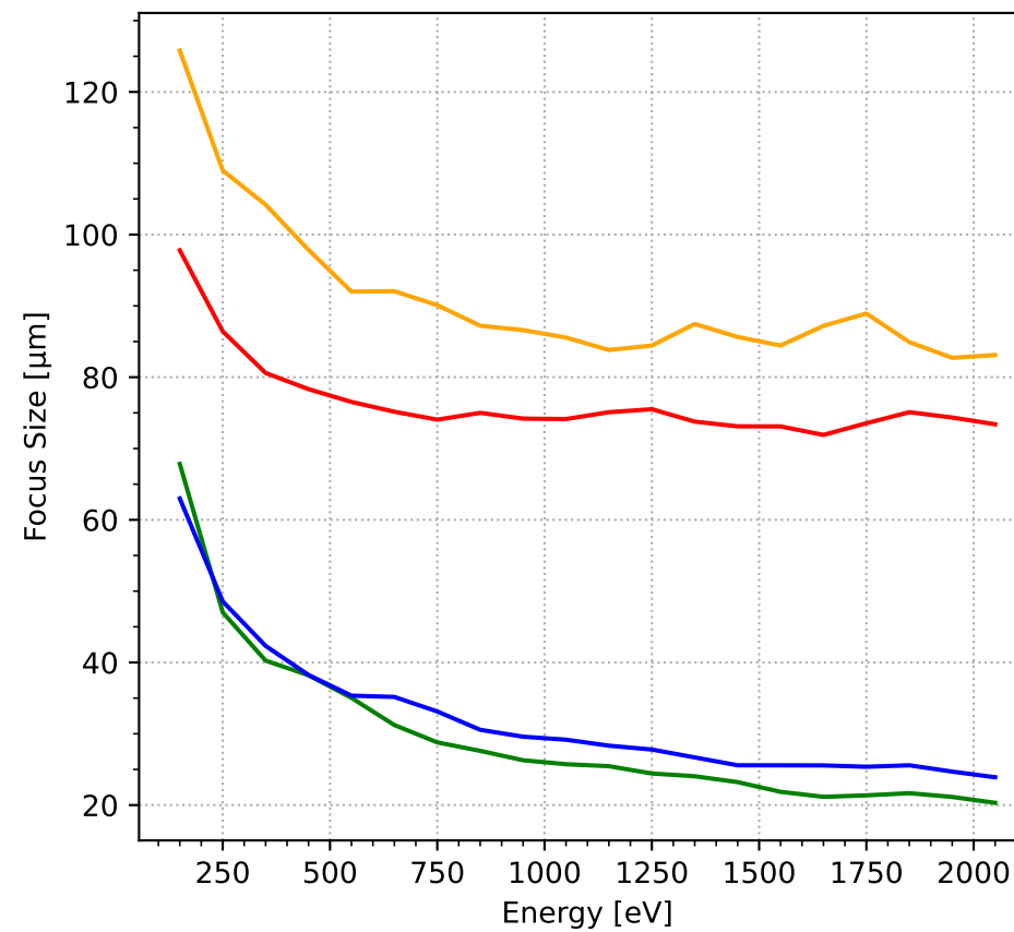
Horizontal Focus
