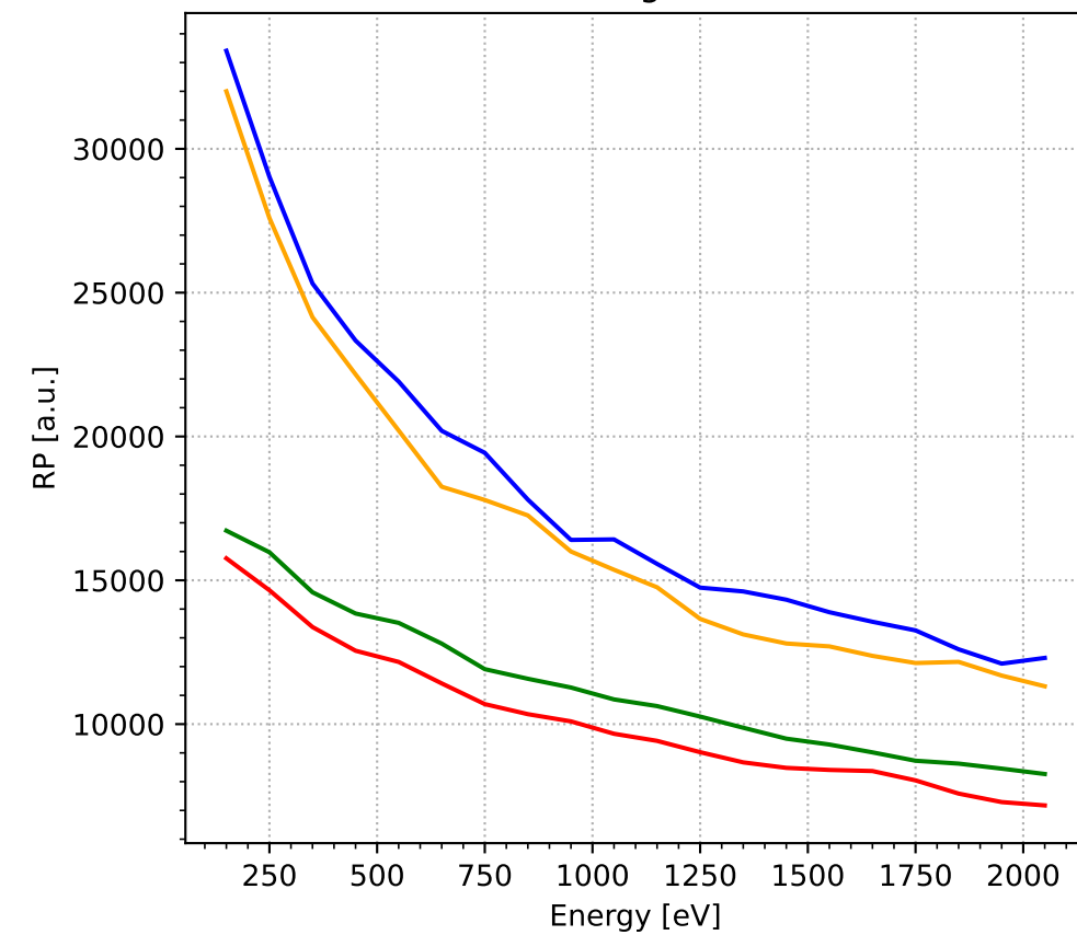
Resolving Power
