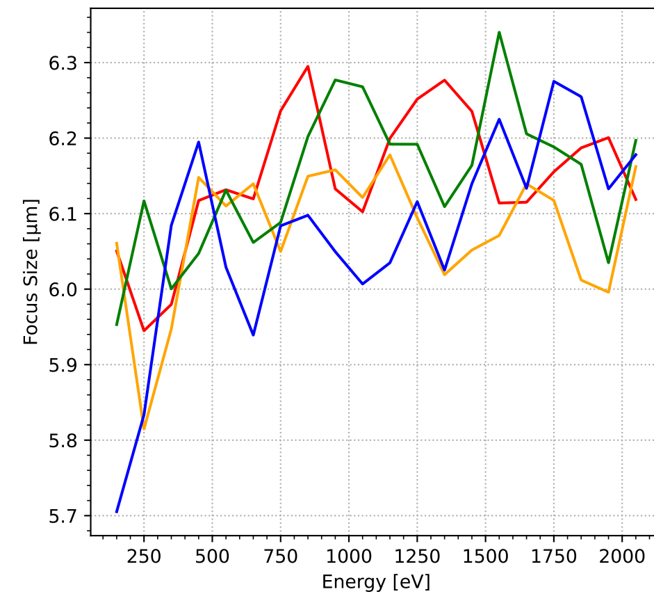
Vertical Focus
