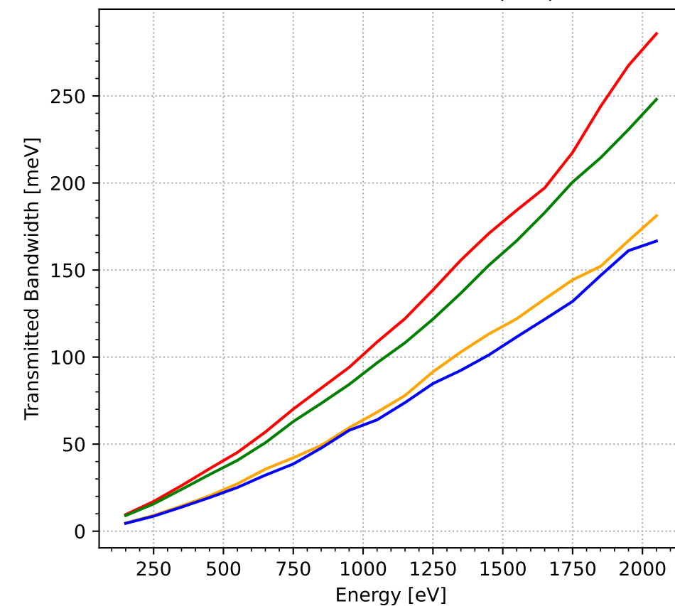
Vertical Focus
